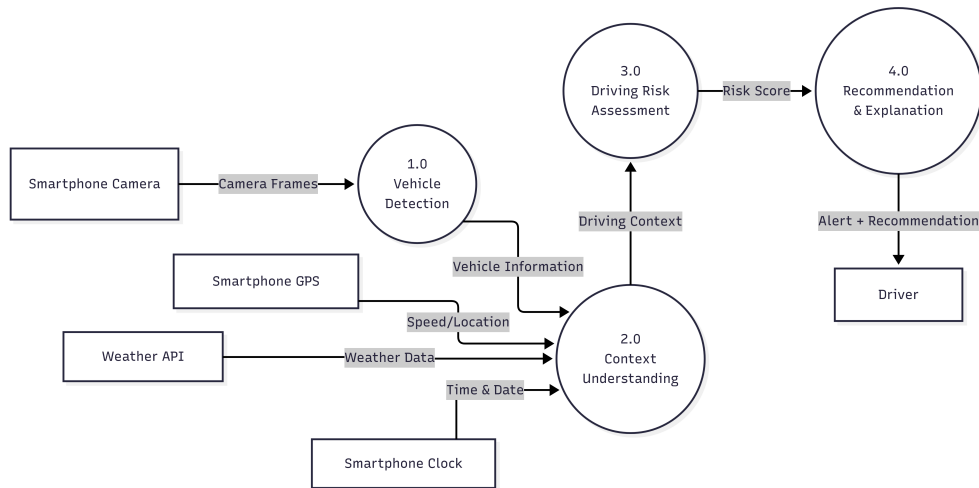
Figure 4.5: Data Flow Diagram - Level 2
