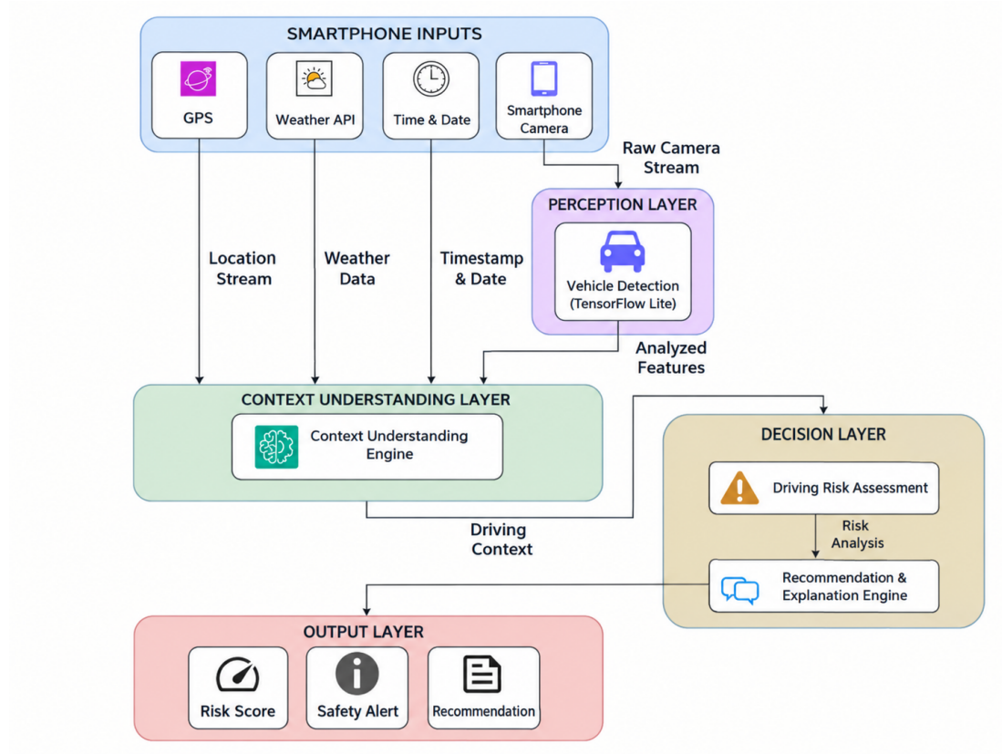
Figure 4.1: Architecture Diagram of ContextDrive
